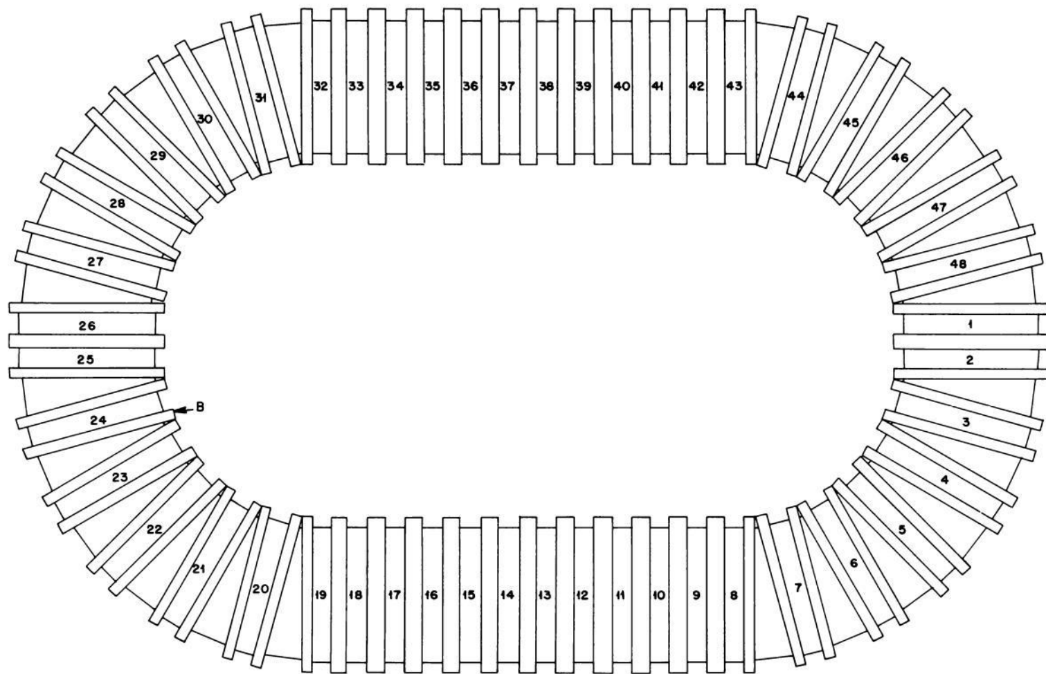
Fig. 3.20—Plan view of magnet model A.
