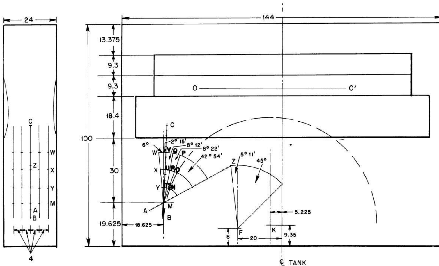
Fig. 2.55—Location of source-region-device measurements in Alpha I.
