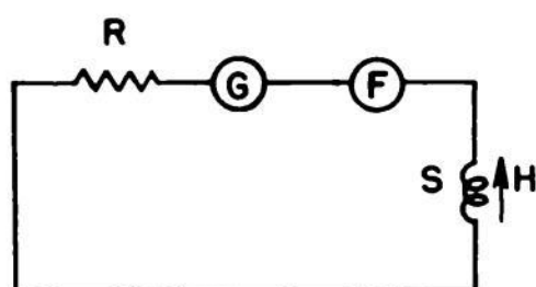
Fig. 2.1 — Ballistic galvanometer circuit.
