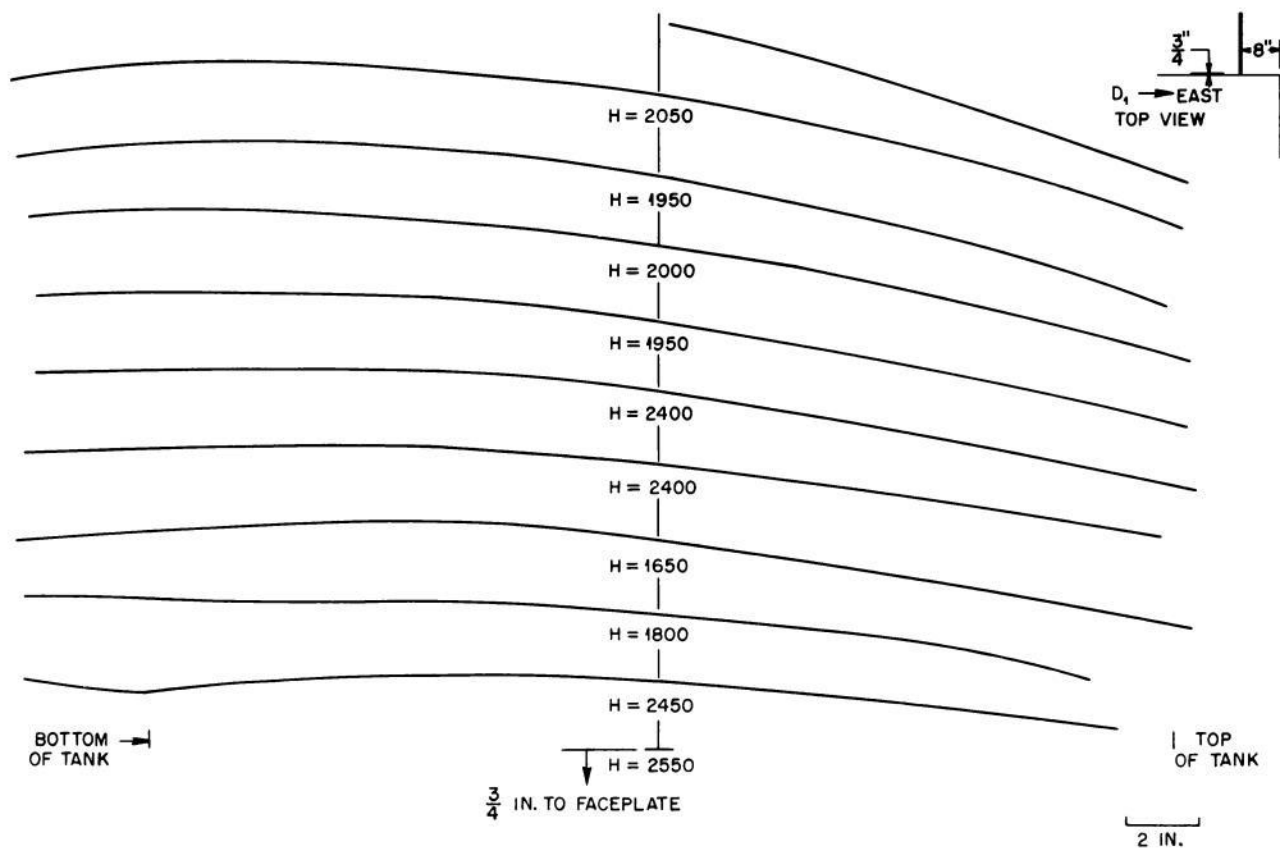
Fig. 4.12—Flux plot for the D_1 tank.
