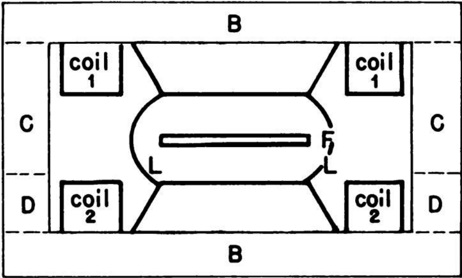
Fig. 1.9 —Alternate design of cyclotron magnet.
