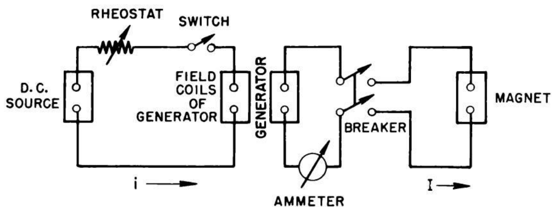
Fig. 2.28—Control circuit used in obtaining magnetization curves.
