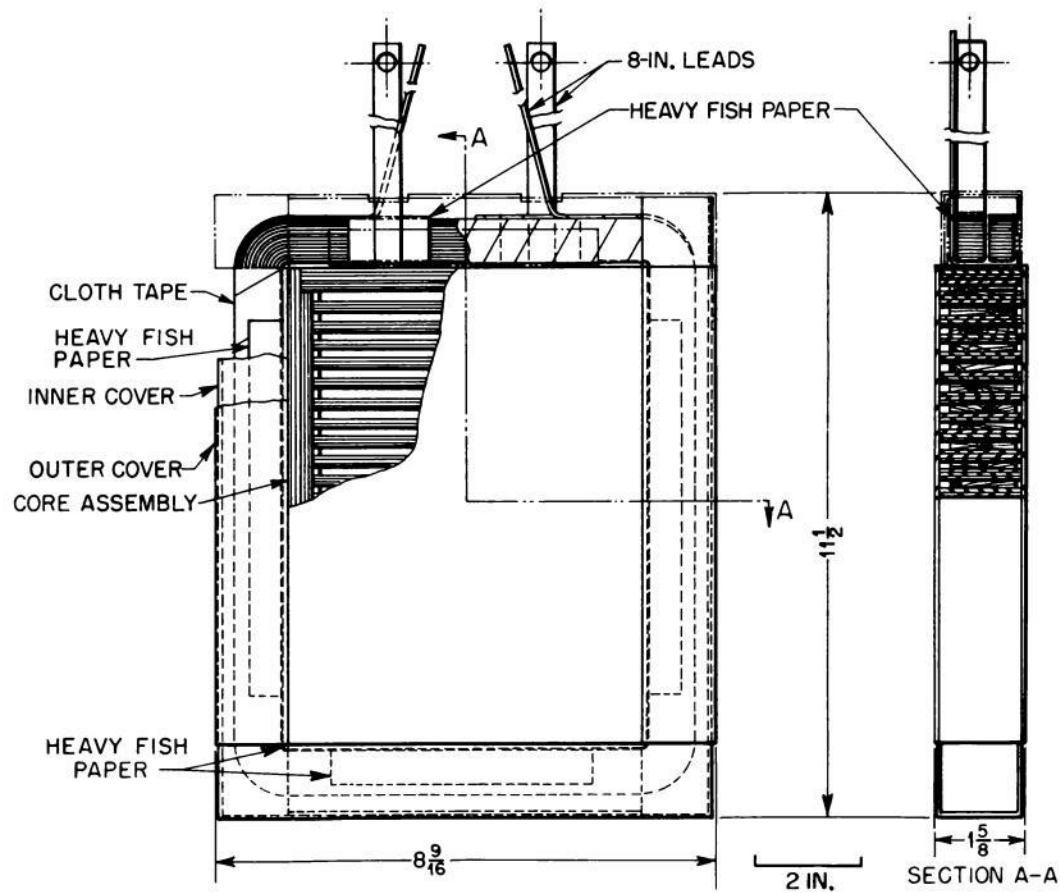
Fig. 3.5—Coil cooling tanks for magnet model Alpha II (revised).
