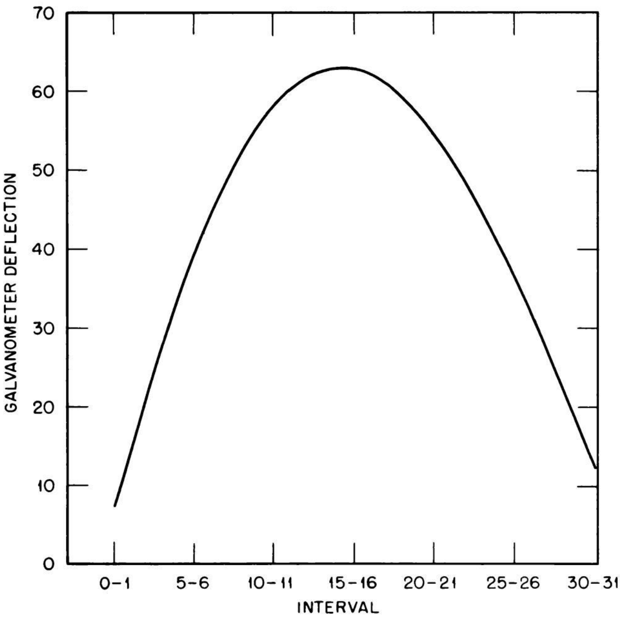
Fig. 2.54—Example of experimental \int h_z \, dx curve.
