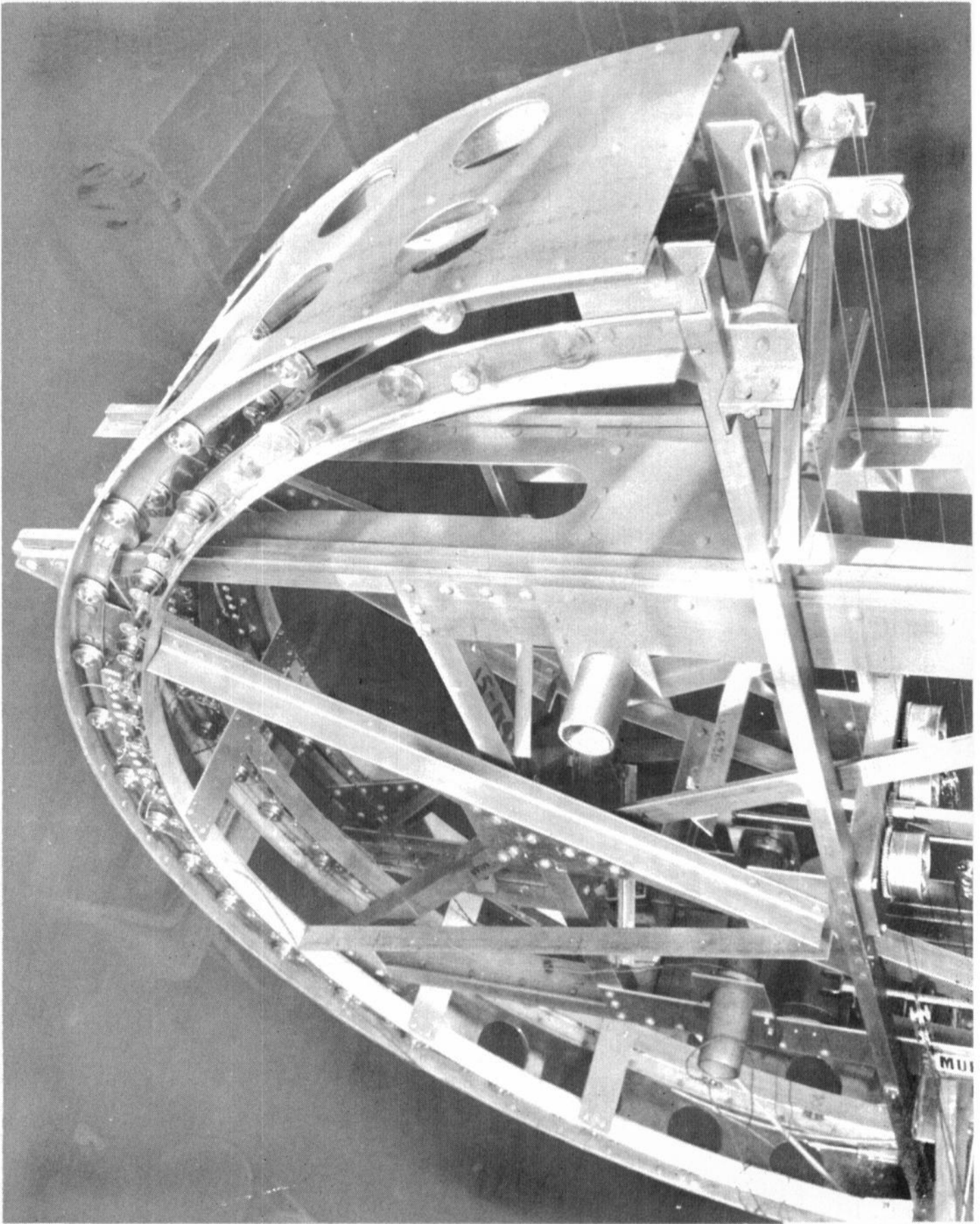
Fig. 2.51 — View of shim device II (magnet 108).
