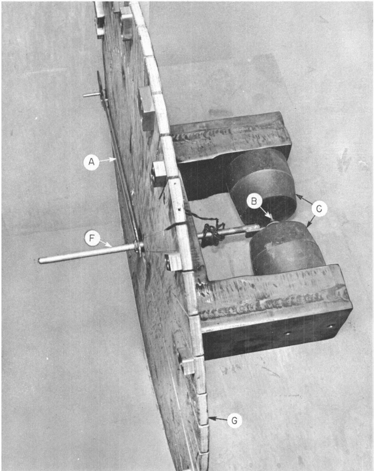
Fig. 2.26b—View of flux standard, type II. Magnet 327.
