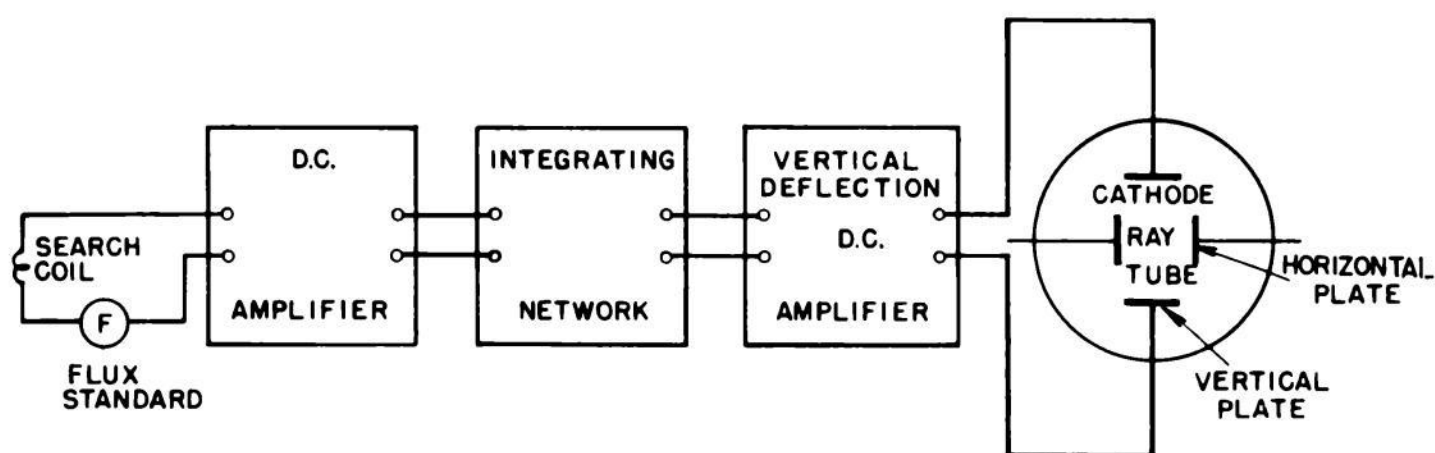
Fig. 2.3 — Circuit for electronic fluxmeter with oscilloscope.
