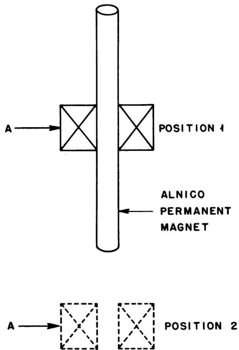
Fig. 2.25—Method of operation of flux standard.
