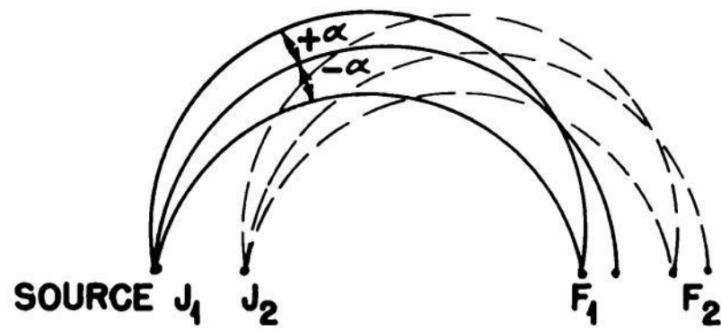
Fig. 1.1 — Ion focuses for uniform magnetic field.
