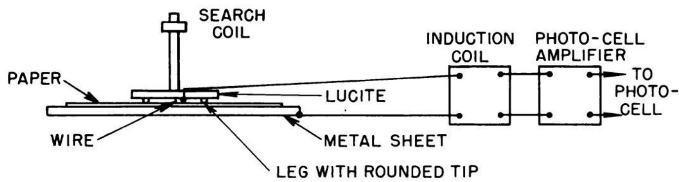
Fig. 2.46—Apparatus for recording points on a contour for contour-mapping device [Fig. 5B of Daily Log (Z Group), Aug. 7, 1944].
