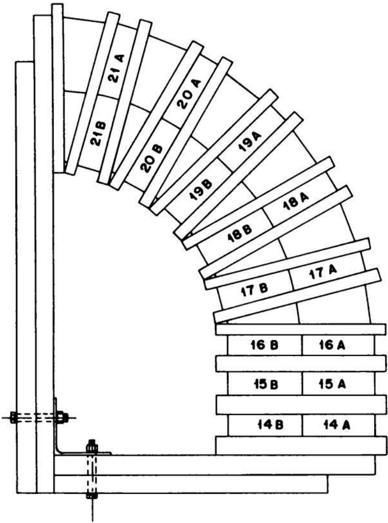
Fig. 3.21—Section of magnet model A.
