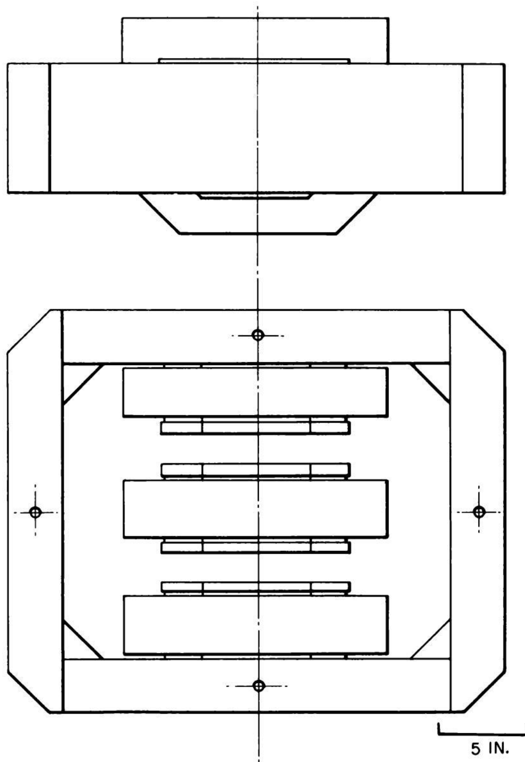
Fig. 1.12 — Scale model of cyclotron magnet.
