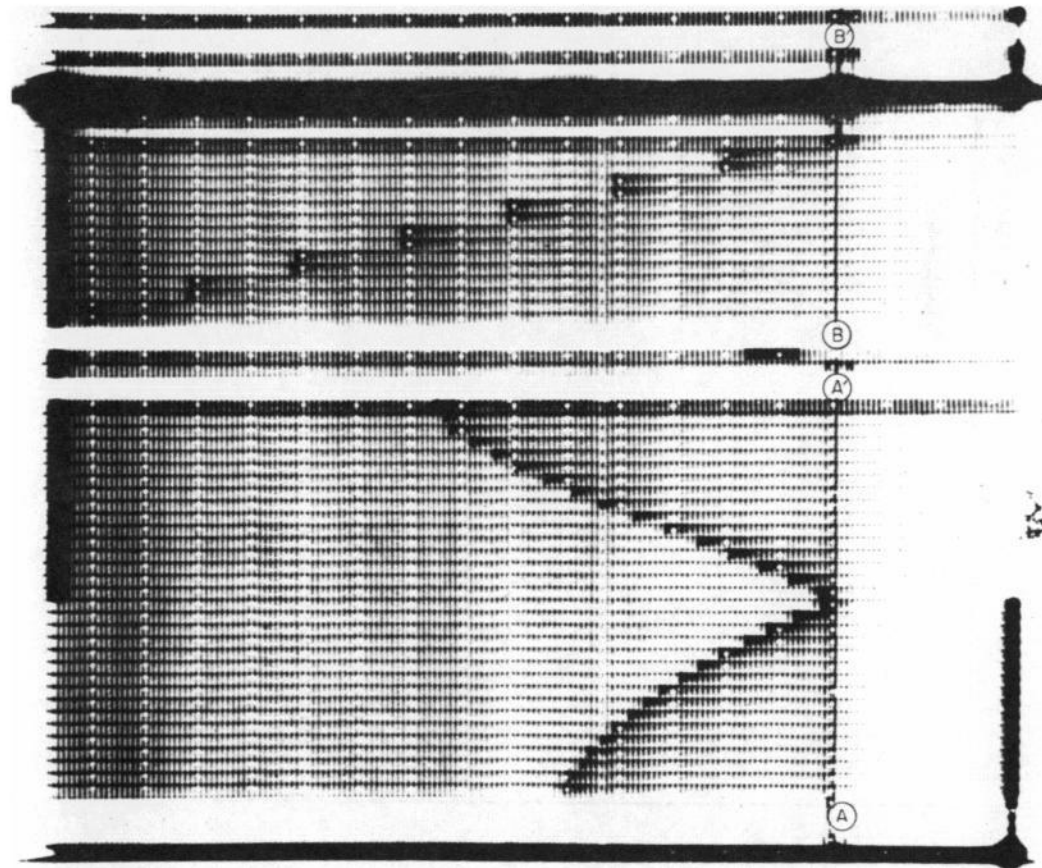
Fig. 2.53—Arc-of-coils photographed data (magnet 350).
