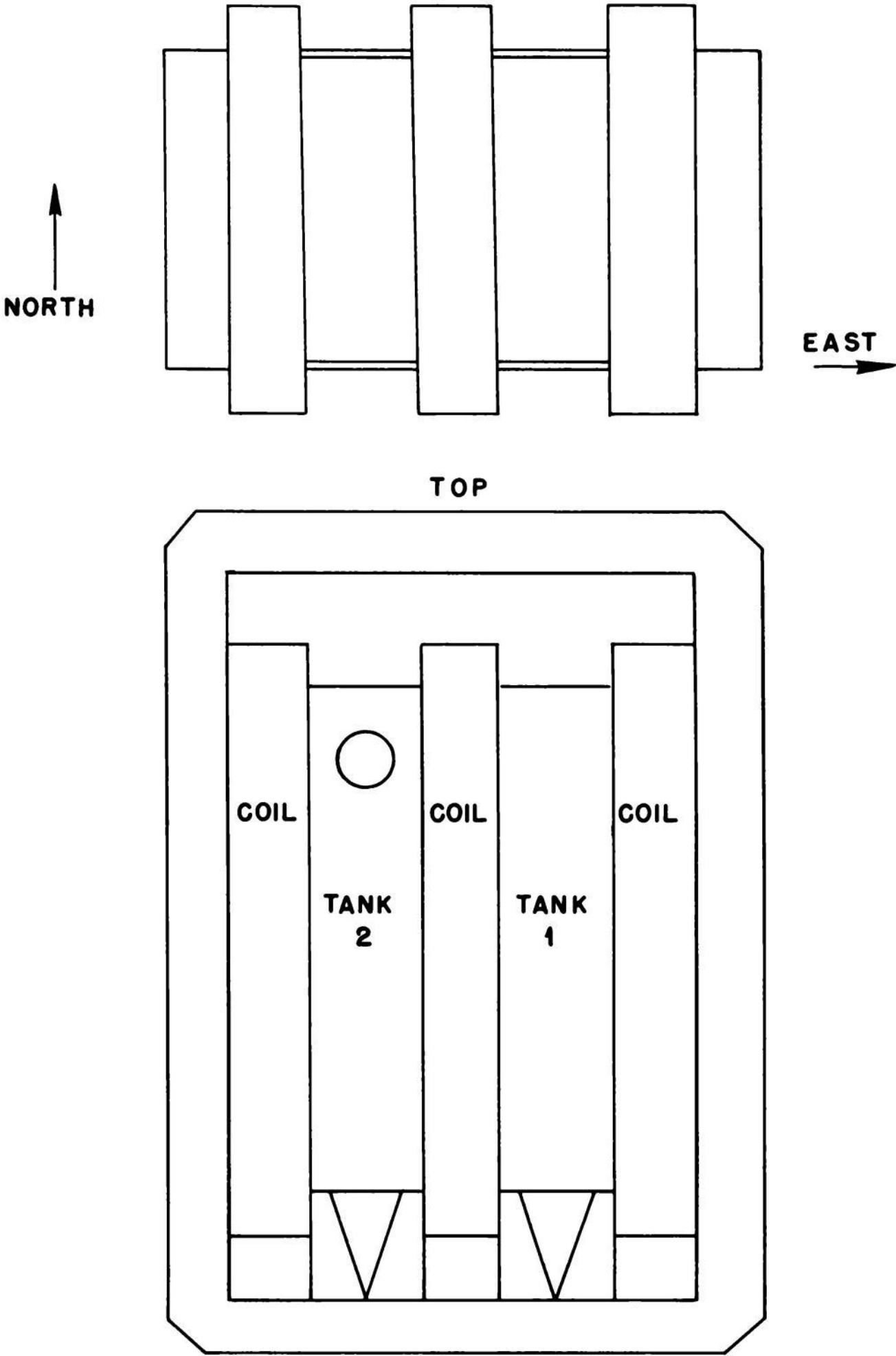
Fig. 4.1 — View of the XA magnet.
