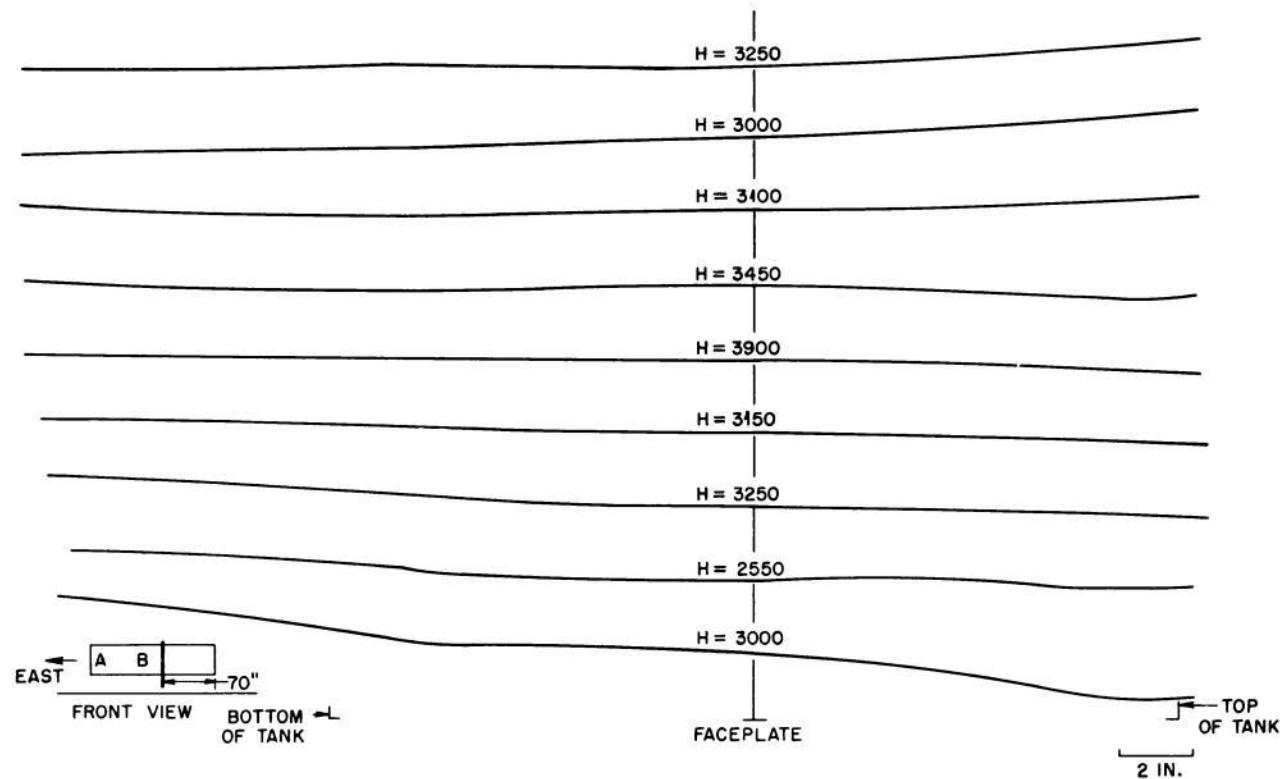
Fig. 4.14 — Flux plot for the R 1 tank.
