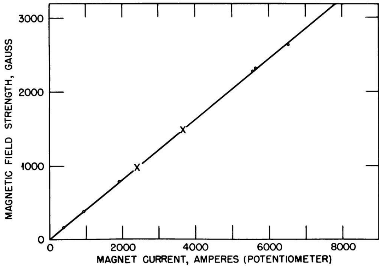
Fig. 4.24—Magnetization curve for tank 89 in race track 1.
