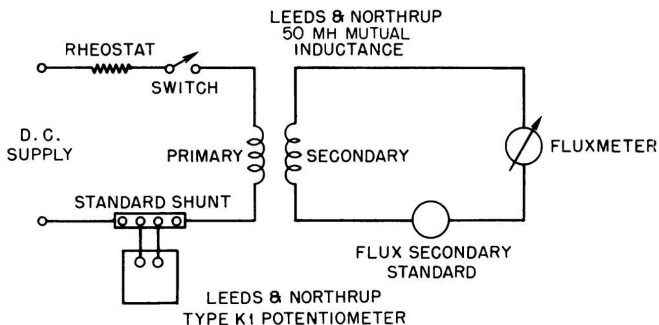
Fig. 2.27—Standardizing circuit for flux standards.
