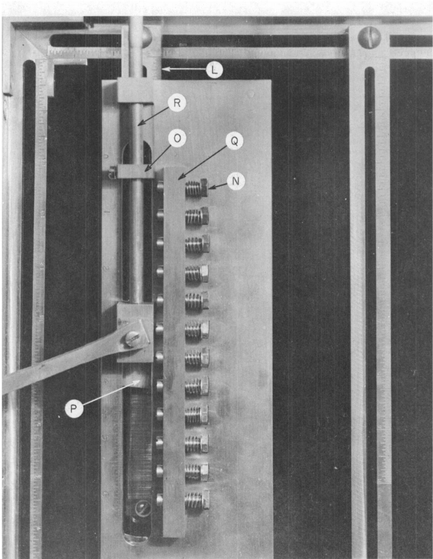
Fig. 2.36 — Close-up of stylus guide (magnet 202).
