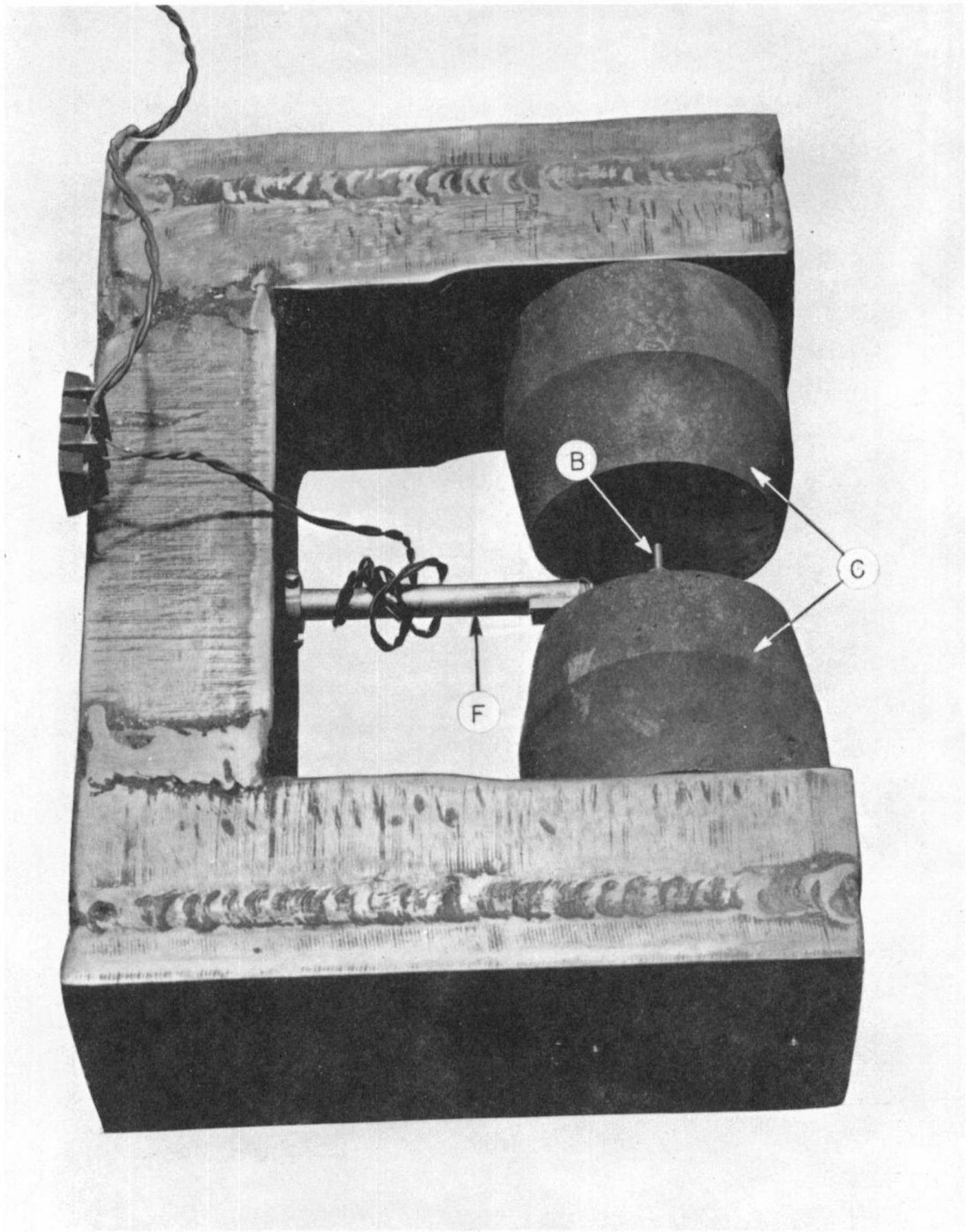
Fig. 2.26a — View of flux standard, type II. Magnet 326.
