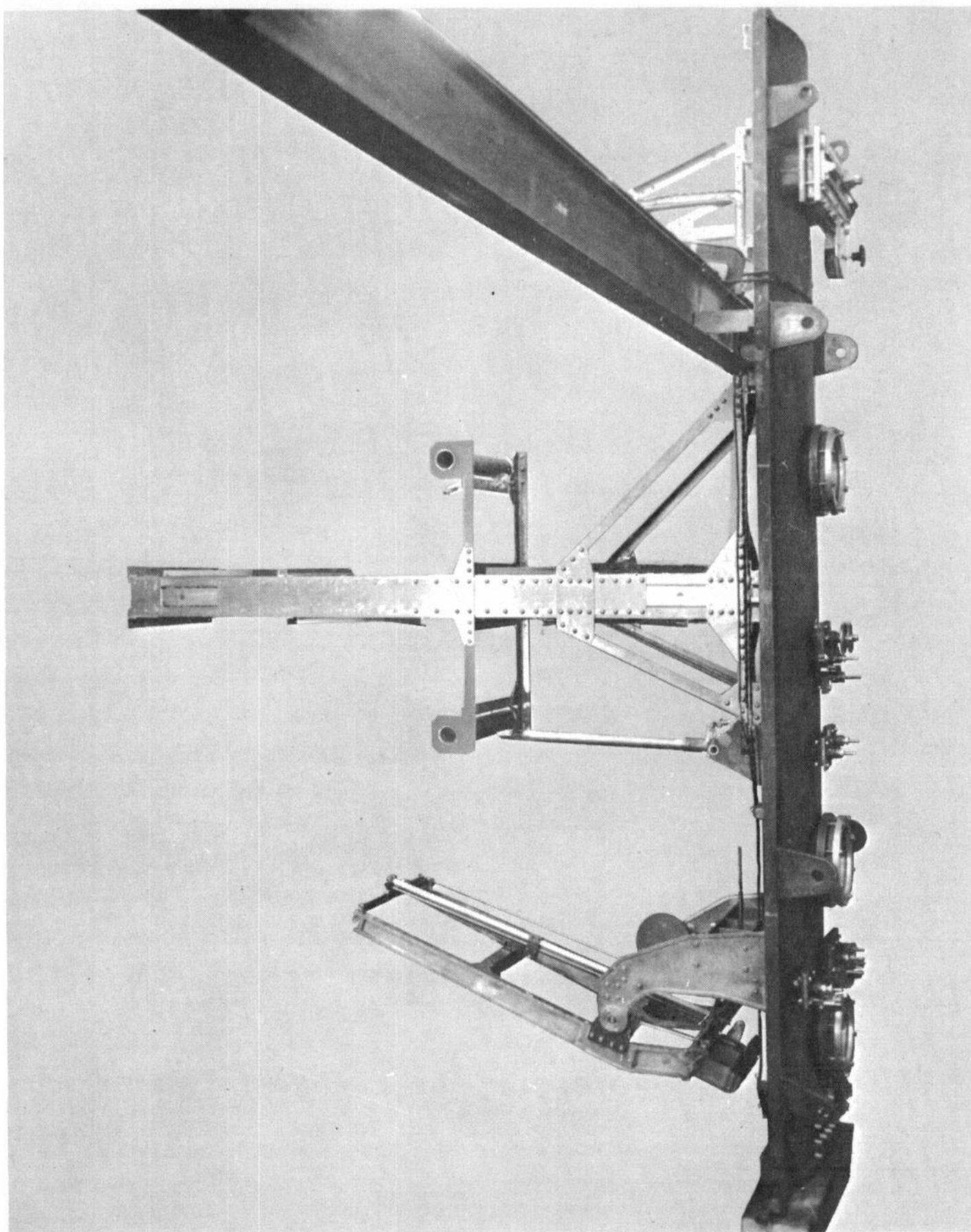
Fig. 2.57 —General view of source-region device (magnet 118).
