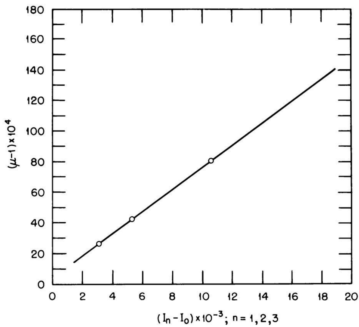
Fig. 2.15—Calibration curve for magnetic balance.
