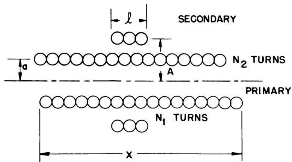
Fig. 2.19— Long solenoid with short secondary outside.
