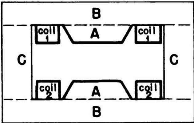
Fig. 1.7 — Cyclotron magnet.
