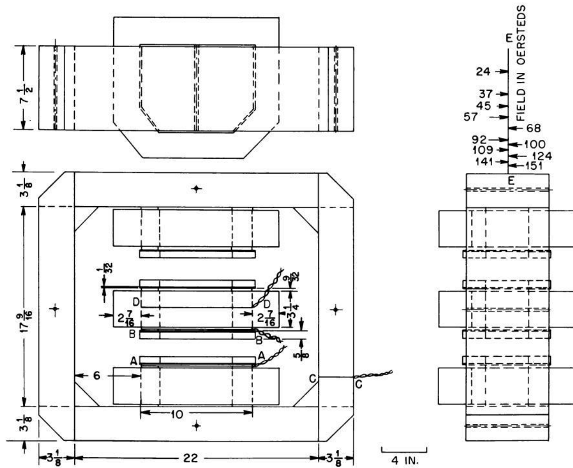
Fig. 3.22—View of magnet model X Beta.
