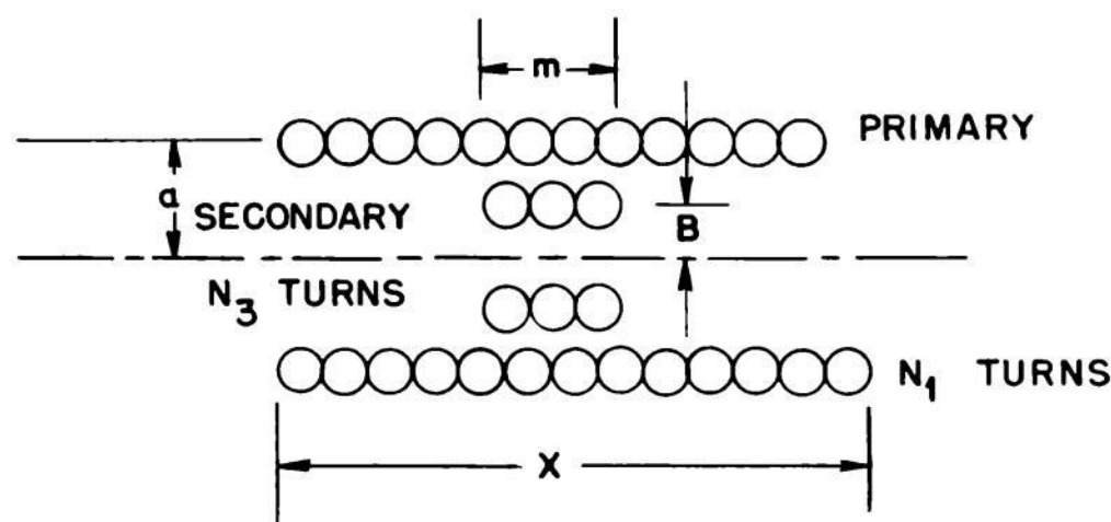
Fig. 2.20— Long solenoid with short secondary inside.
