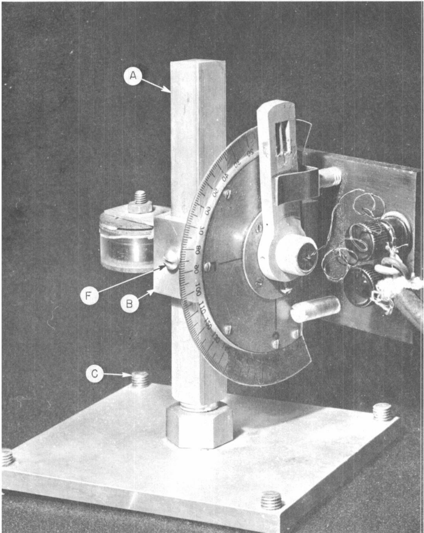
Fig. 2.32 — Flip-coil mount, type II (magnet 323).
