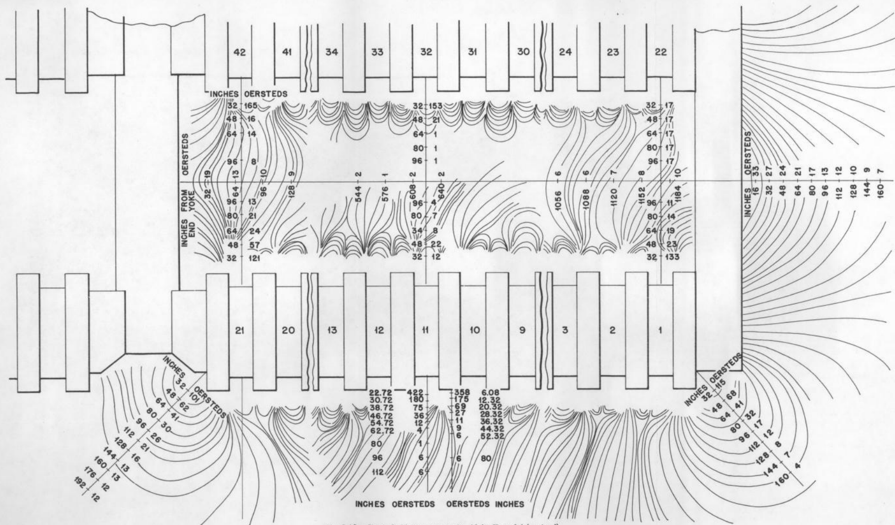
Fig. 3.18—Stray-field measurements, Alpha II model (revised).
