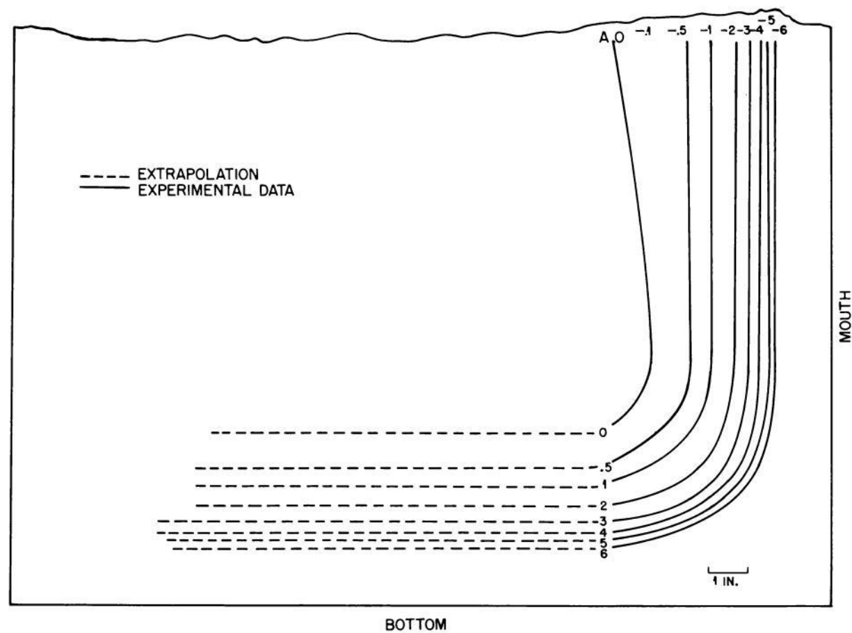
Fig. 4.26—Contour map for tank 84, race track 6.
