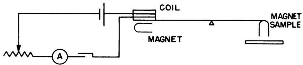
Fig. 2.13—Principle of operation of balance.
