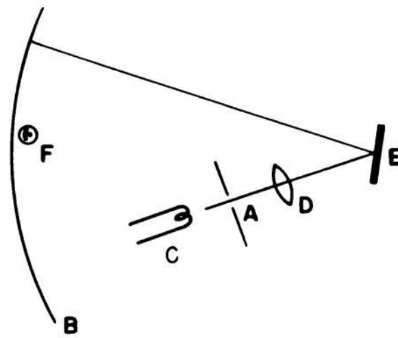
Fig. 2.44 — Optical system for contour-mapping device.
