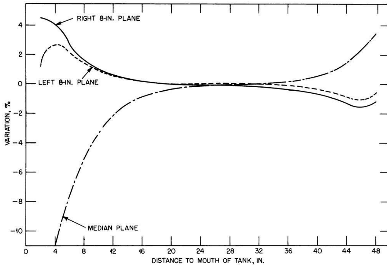
Fig. 4.25—Field distribution in tank 96, race track 6.
