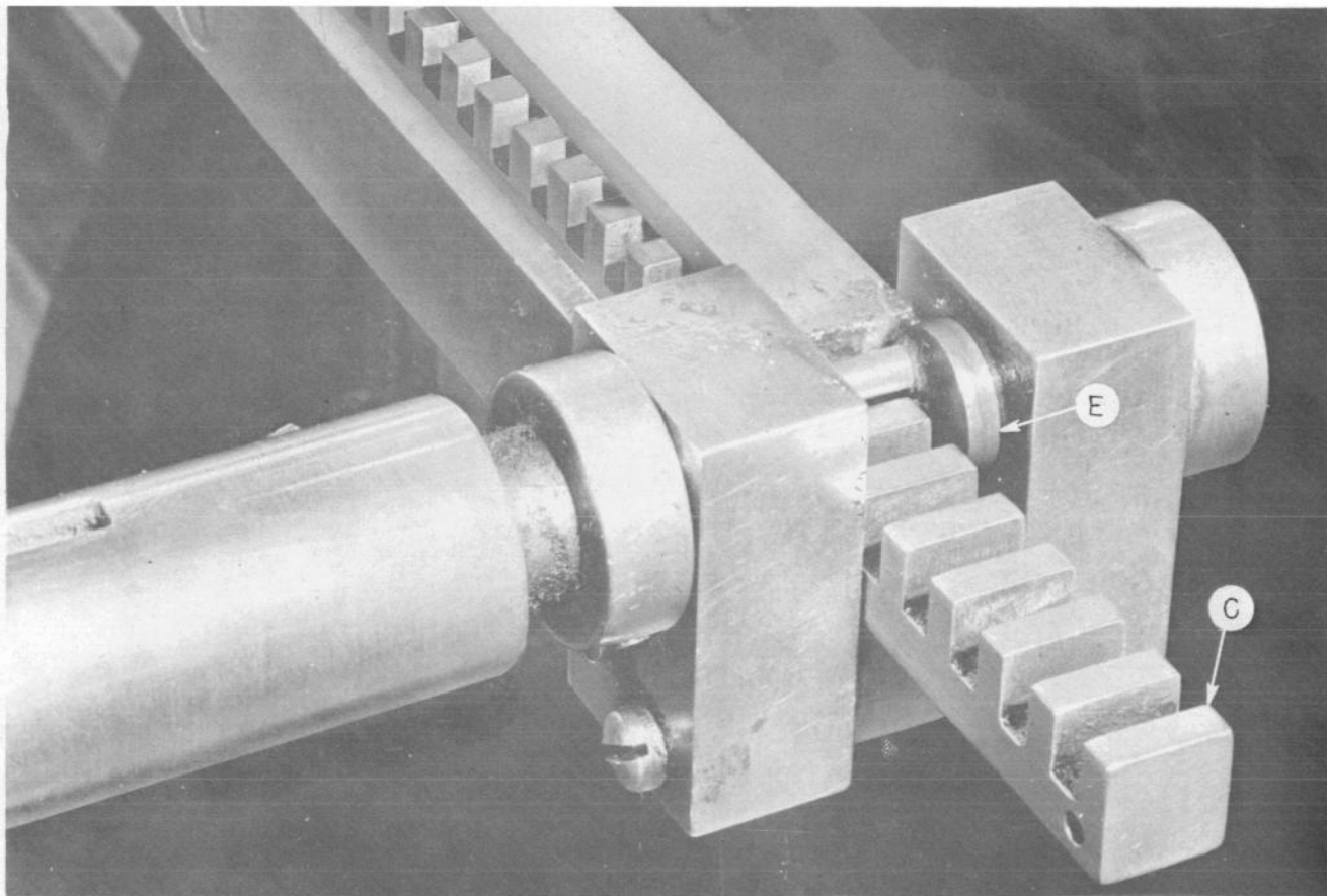
Fig. 2.40—Details of rack and pinion in G.E. fluxmeter method (magnet 318).
