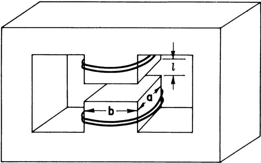
Fig. 1.6 — Magnet used in magnetic force considerations.
