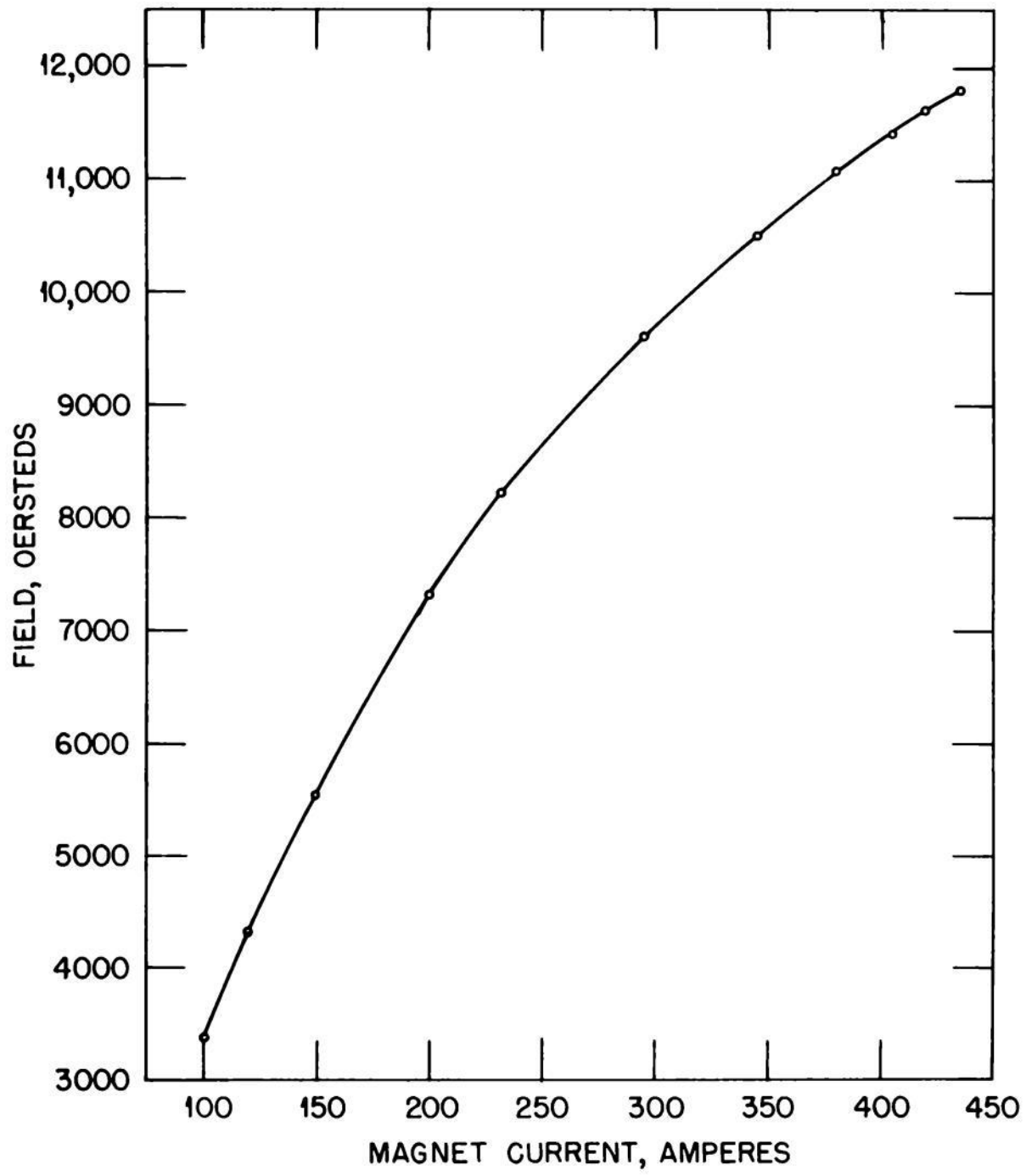
Fig. 4.16—Magnetization curve for the 37-in. cyclotron magnet.
