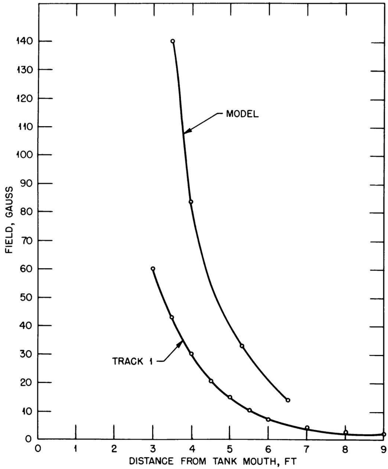
Fig. 4.21 — Stray magnetic field outside tank 43 (race track 1).
