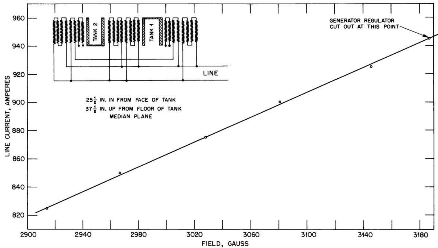
Fig. 4.2—Magnetization curve for the XA magnet.
