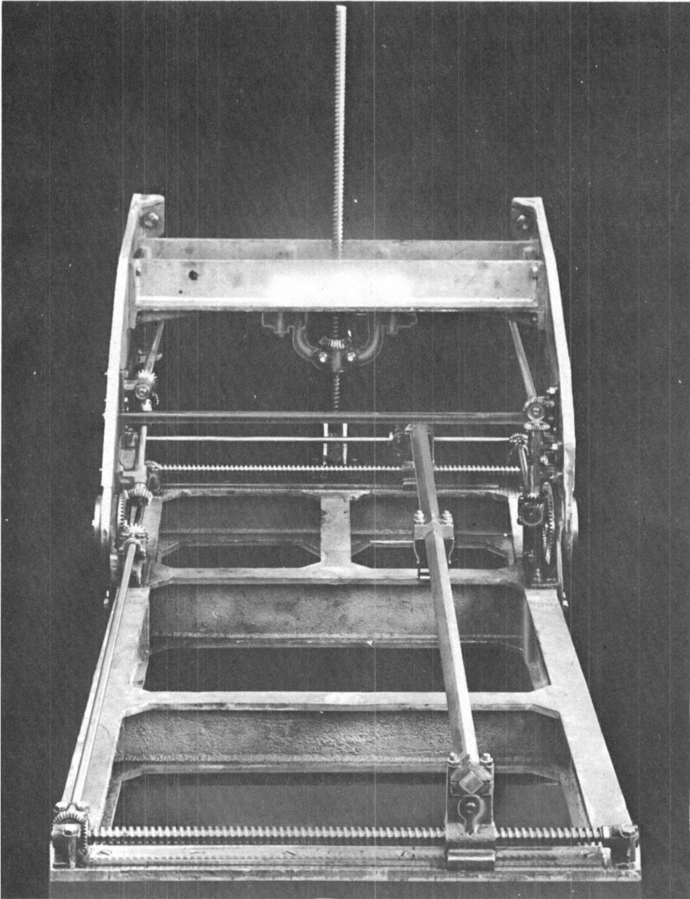
Fig. 2.58—Close-up of portion of source-region device (magnet 76).
