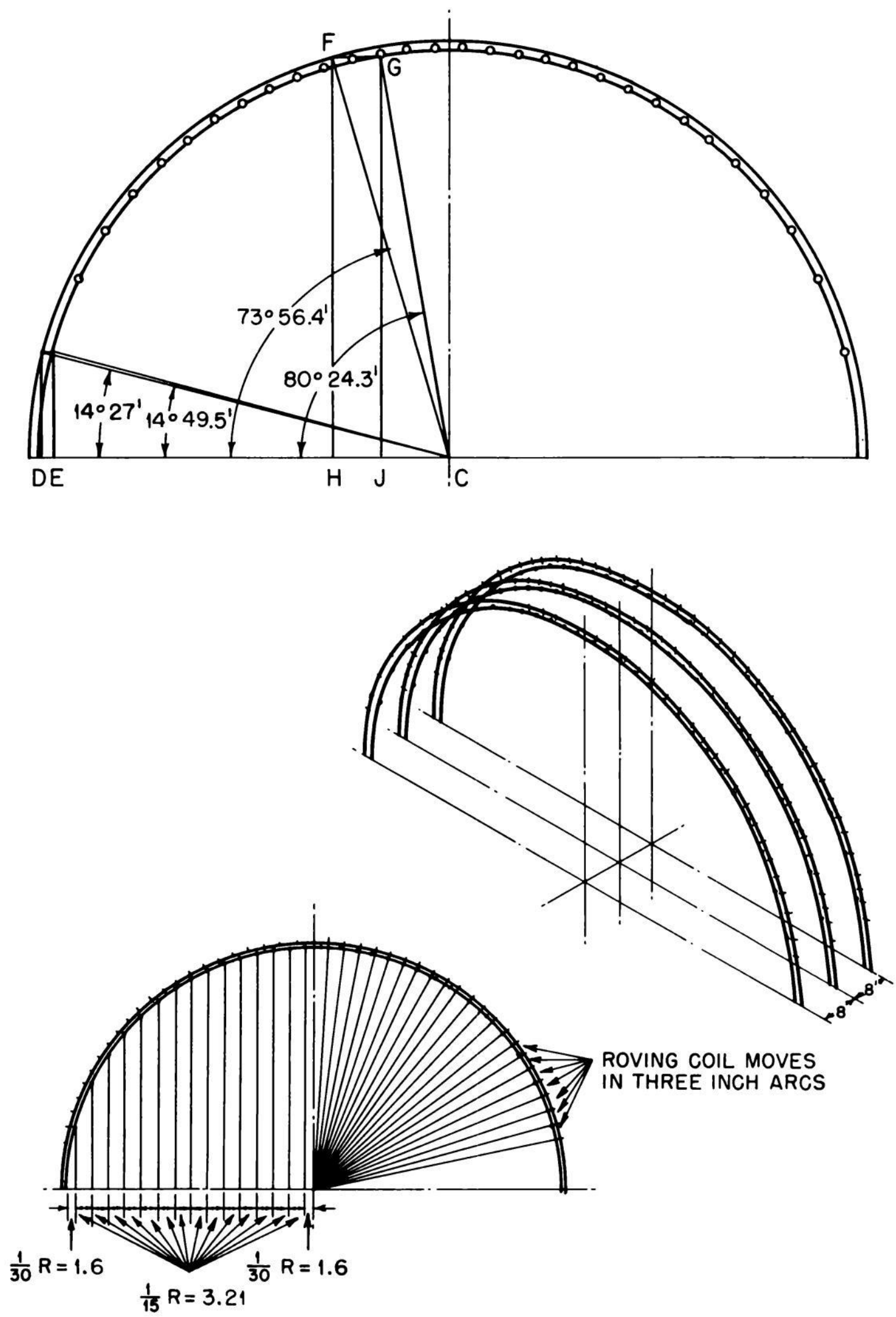
Fig. 2.52— Location of roving-coil measurements.
