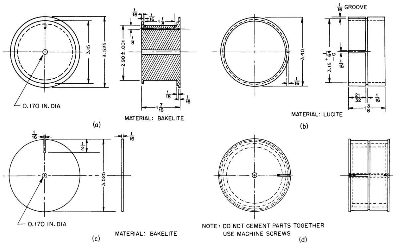
Fig. 2.17—Parts and assembly of standard search-coil form.
