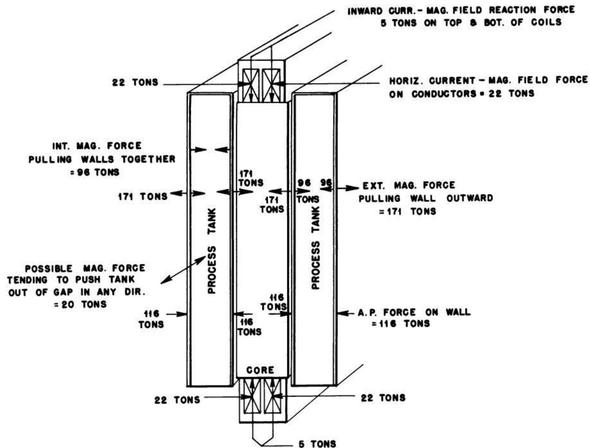
Fig. 3.17— Forces on magnet, magnet model Alpha II (revised).
