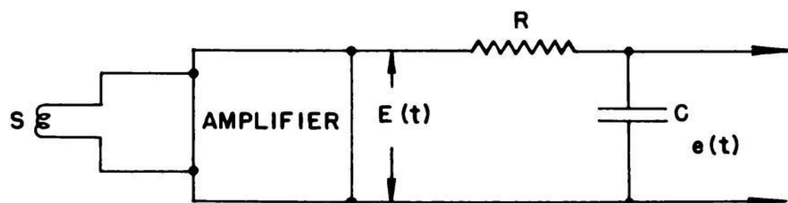
Fig. 2.2 — Basic circuit for electronic fluxmeter.
