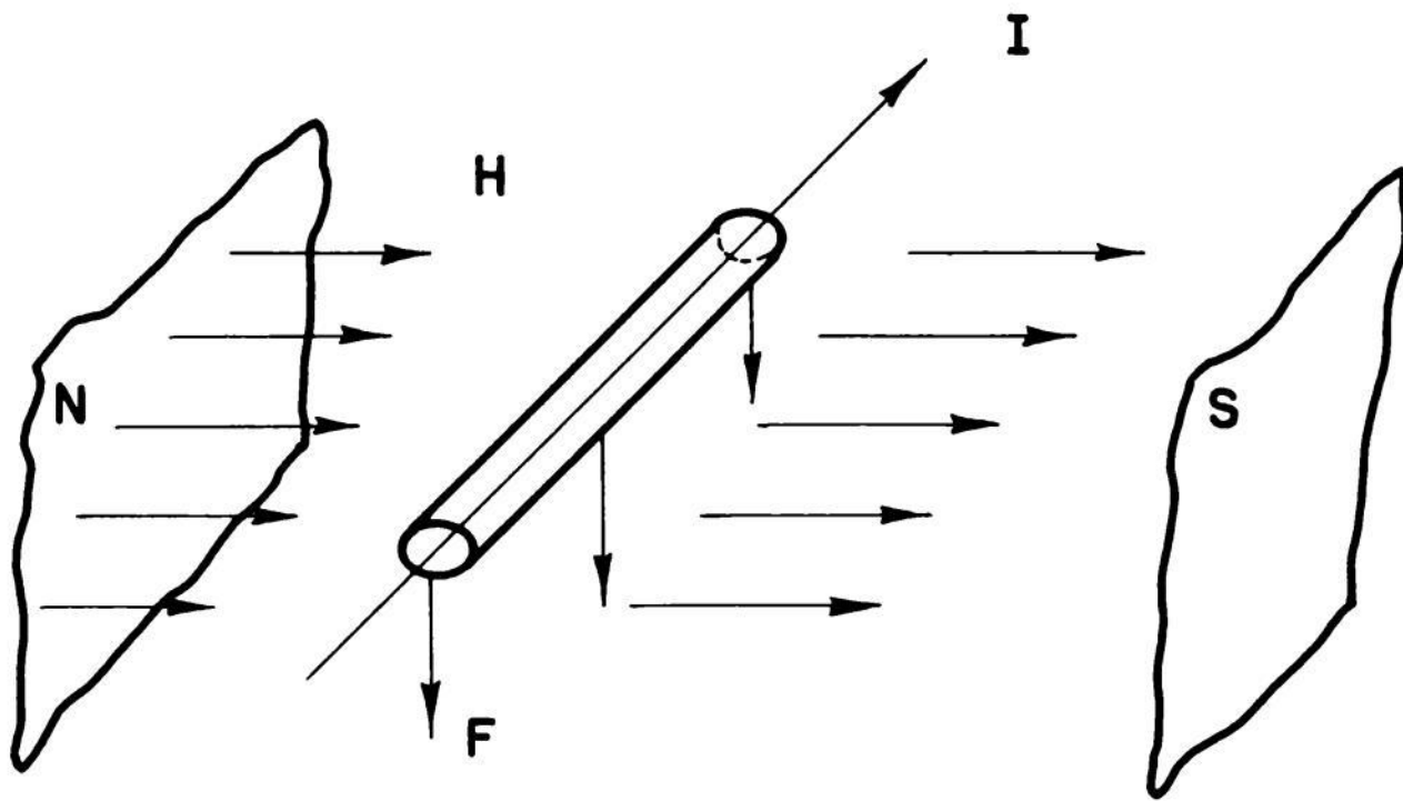
Fig. 1.4 — Force on current-carrying conductor in magnetic field.
