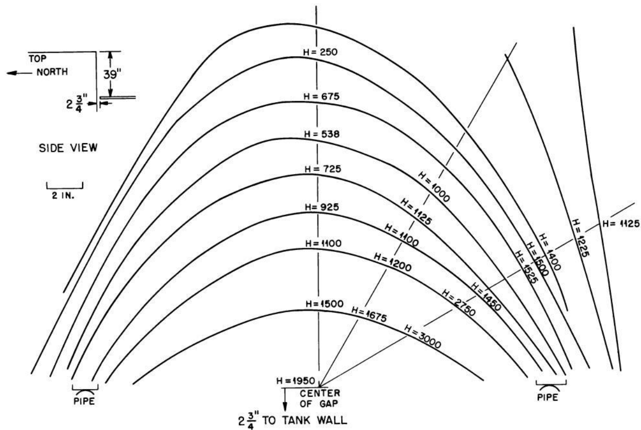
Fig. 4.3—Stray-flux plot around the XA magnet.
