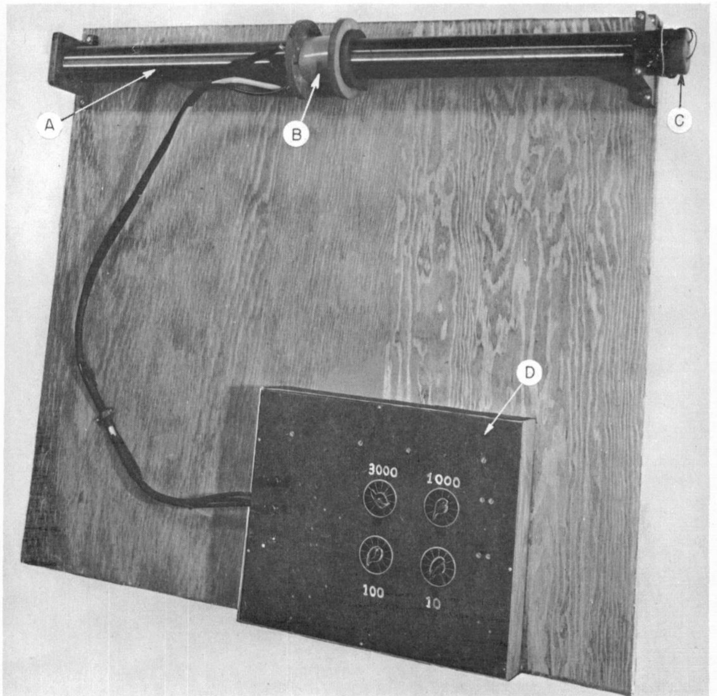
Fig. 2.21 — General view of apparatus involving use of long solenoid to calibrate search coils (magnet 196).
