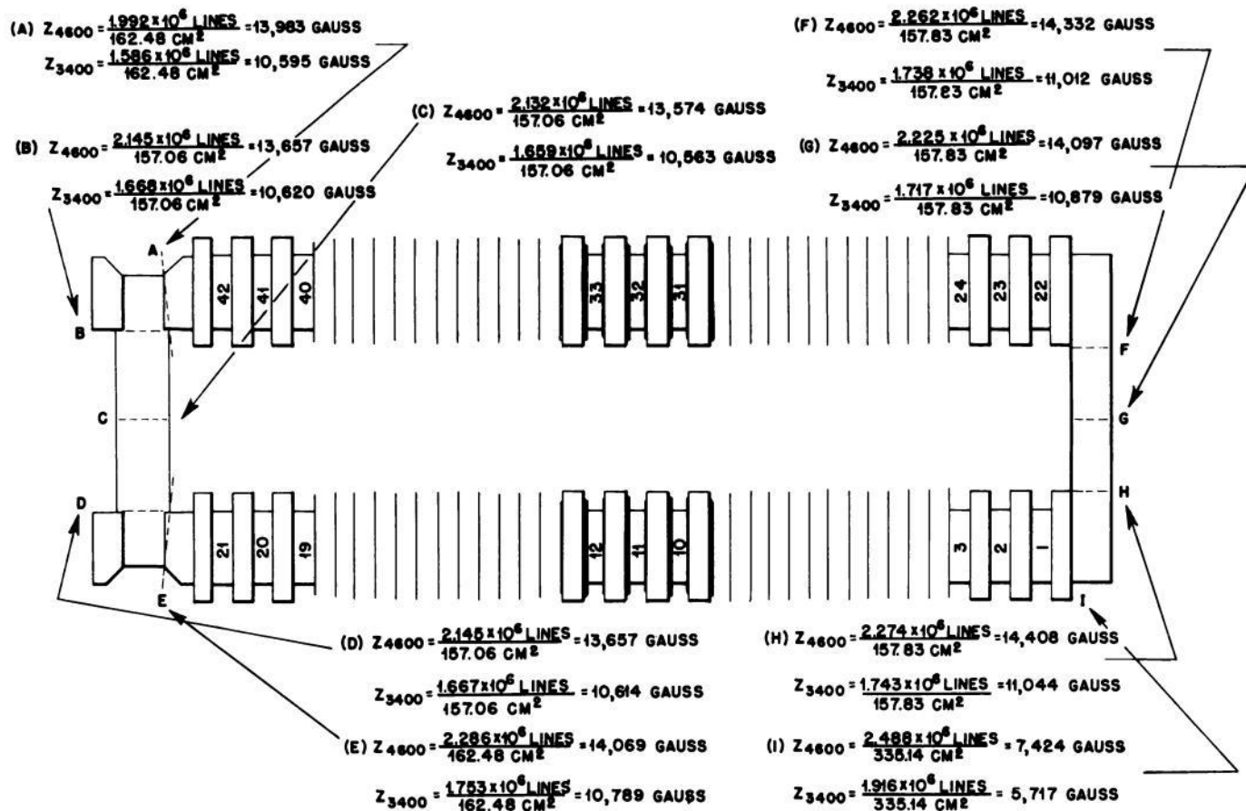
Fig. 3.12—Flux measurements in magnet model Alpha II (revised), case I.
