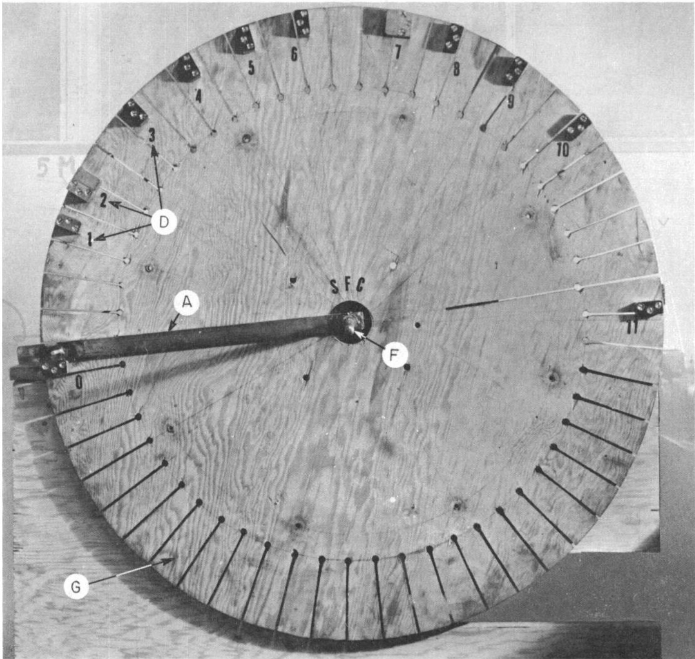
Fig. 2.26c —View of flux standard, type II. Magnet 325.
