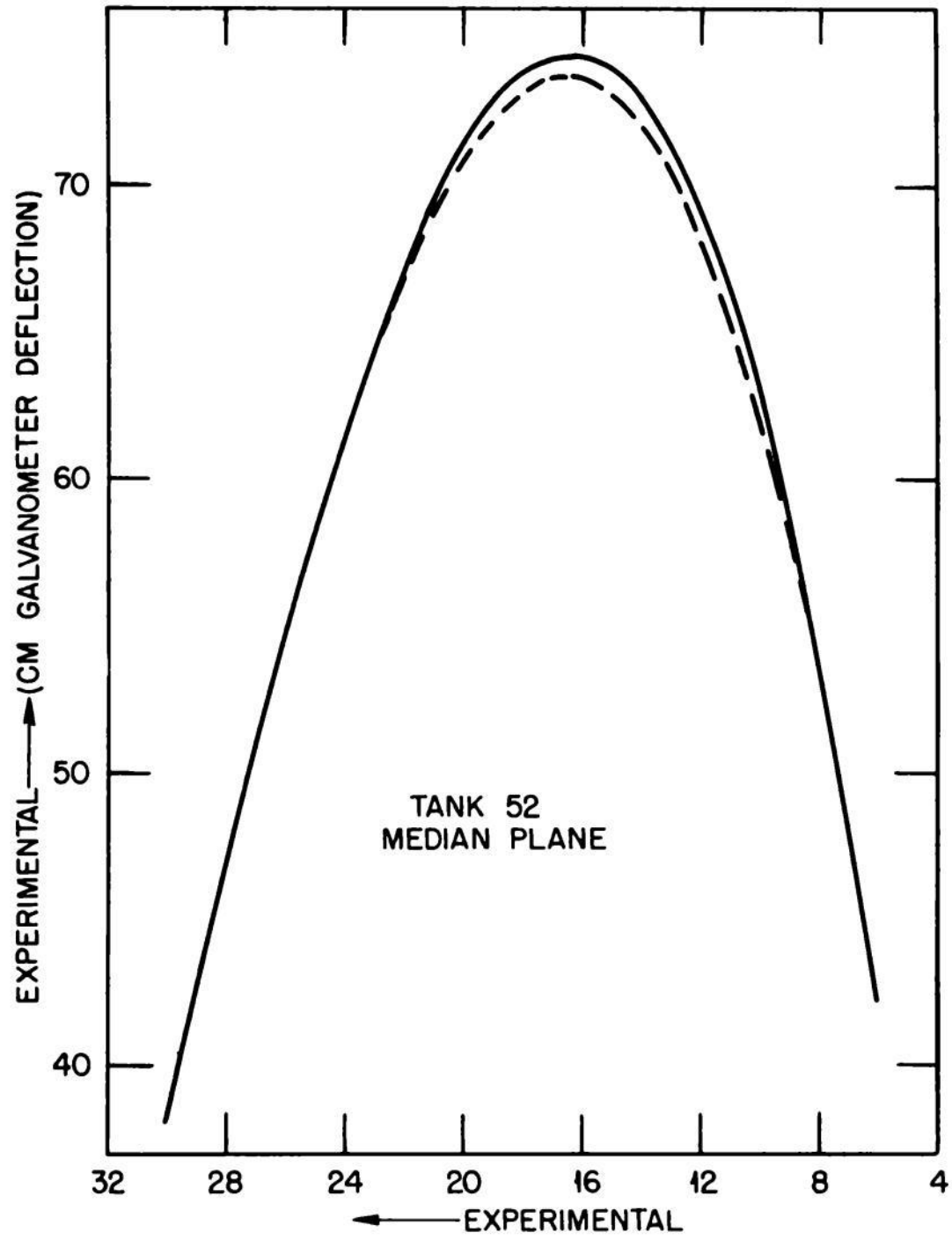
Fig. 4.19—Flattening of peak for curve in median plane, tank 52.
