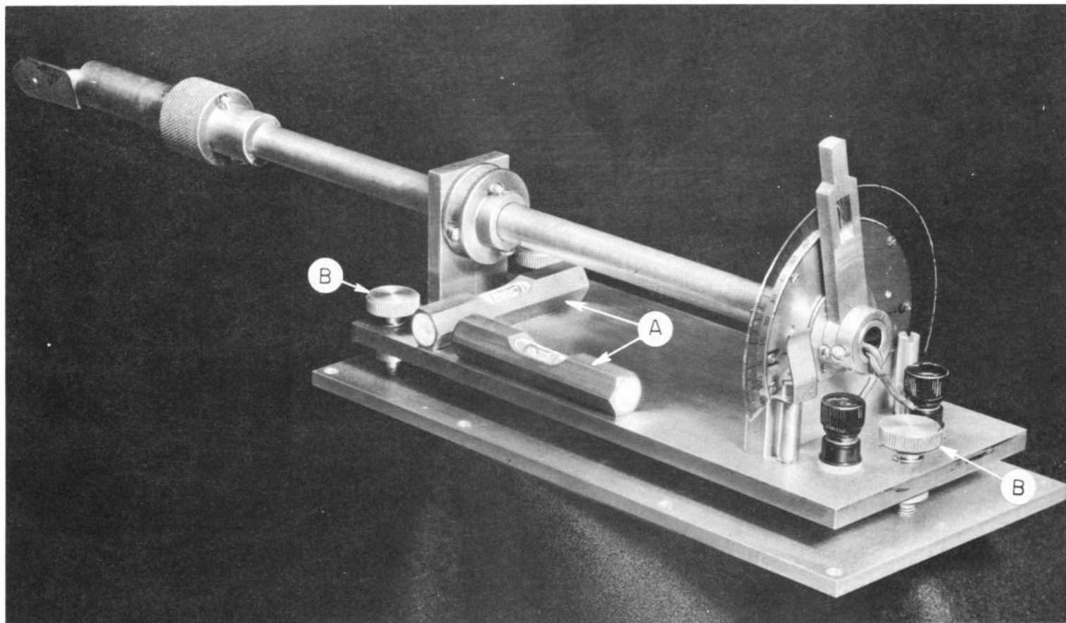
Fig. 2.31 — Flip-coil mount, type I (magnet 203).
