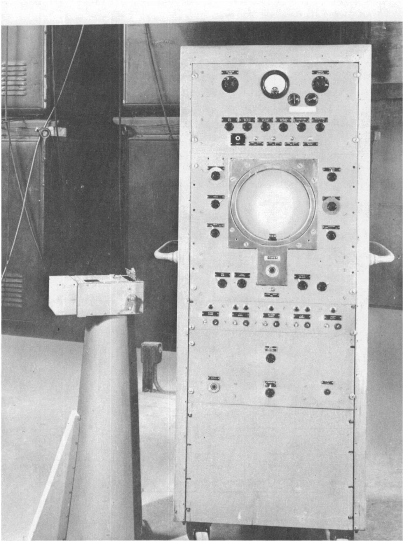
Fig. 2.4—Electronic fluxmeter with 9-in. cathode-ray tube (magnet 336).
