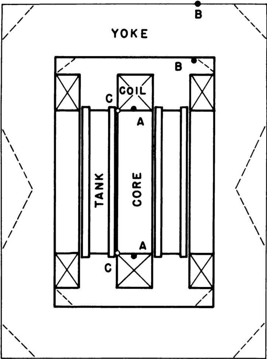
Fig. 1.11 —Schematic drawing of entire cyclotron magnet.
