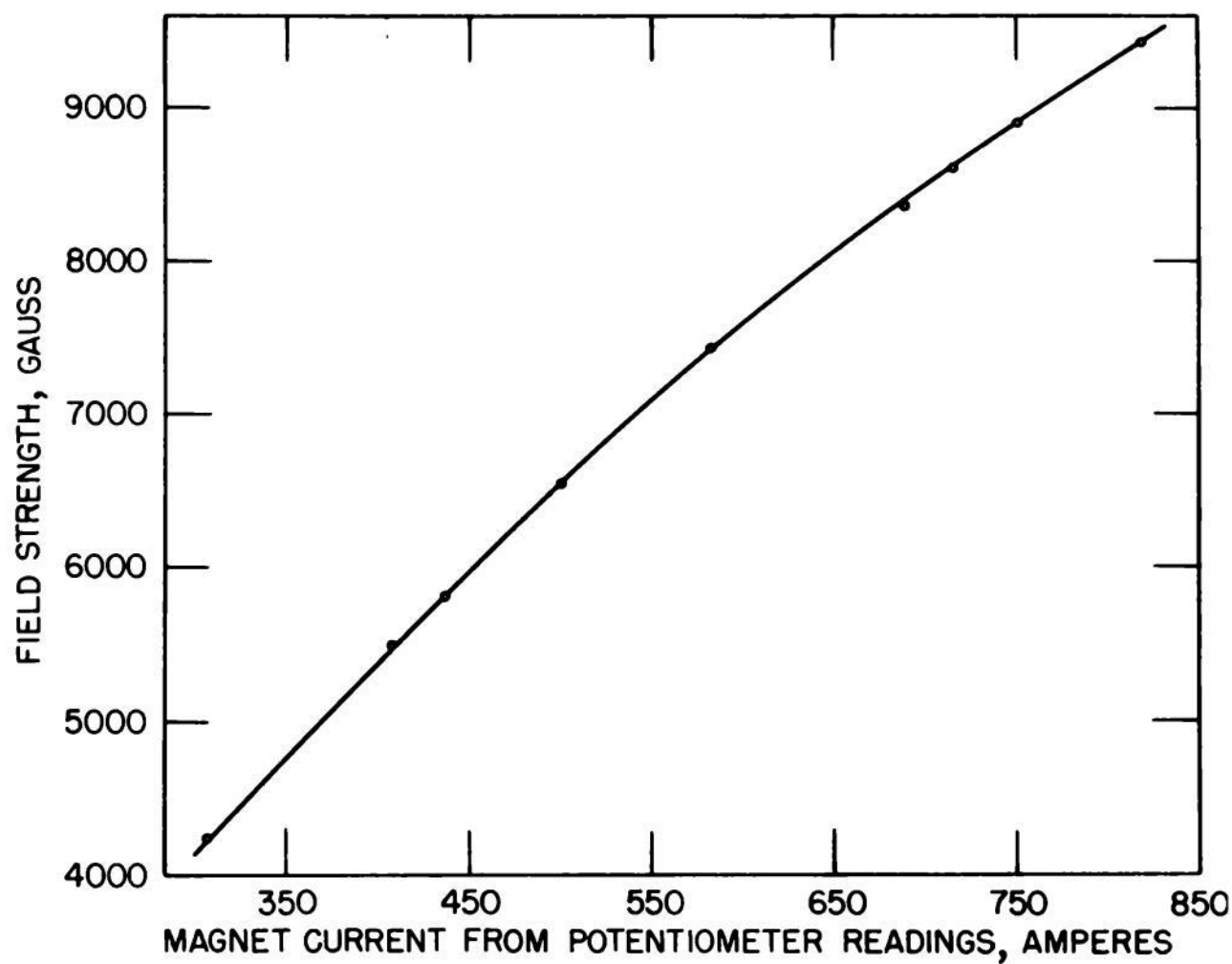
Fig. 4.27—Magnetization curve for magnet XBX.
