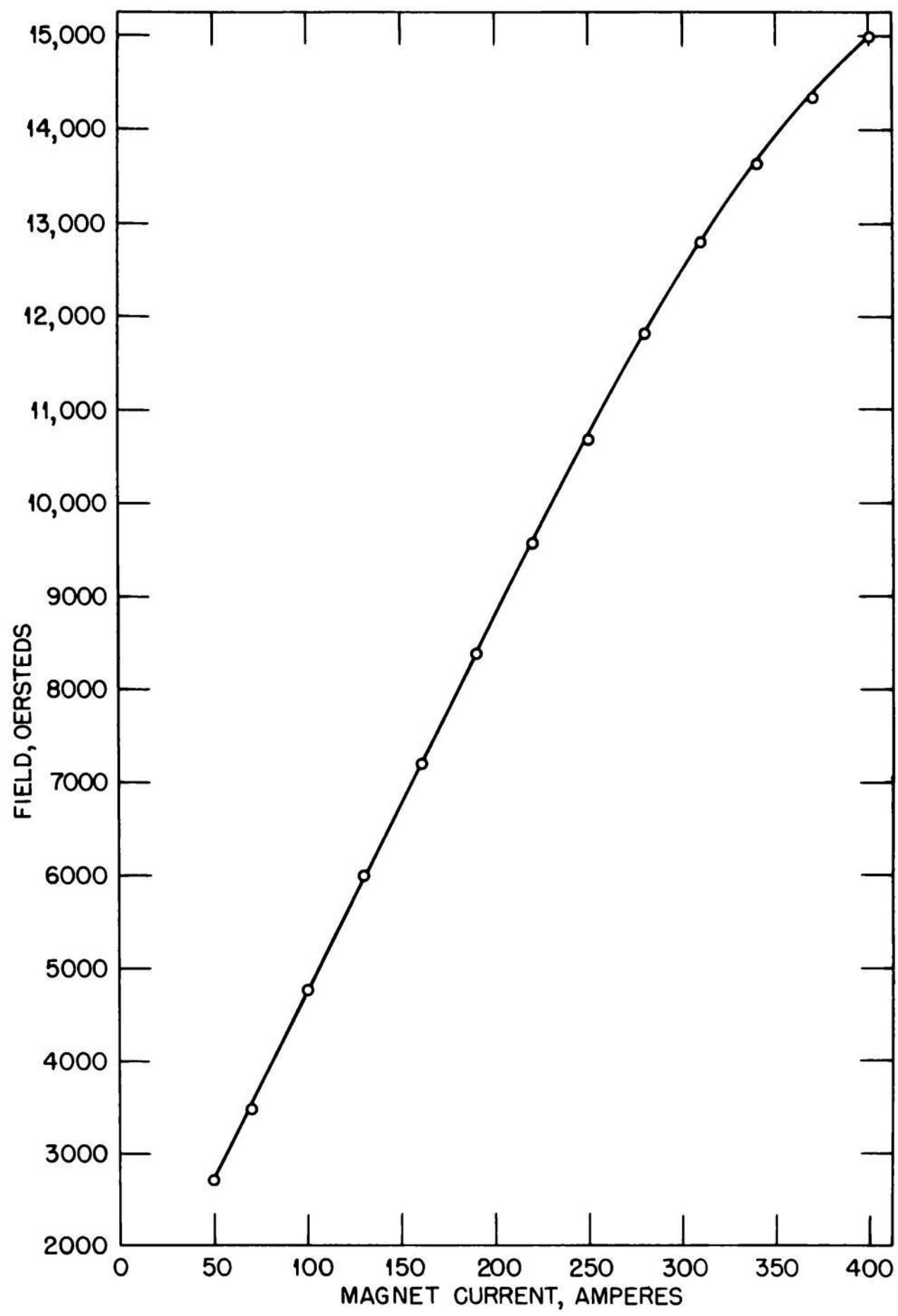
Fig. 4.17 — Magnetization curve for the 60-in. cyclotron magnet.
