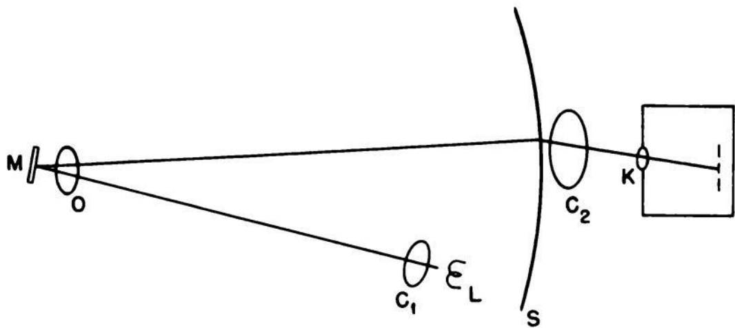
Fig. 2.8—Optical system for fluxmeter.
