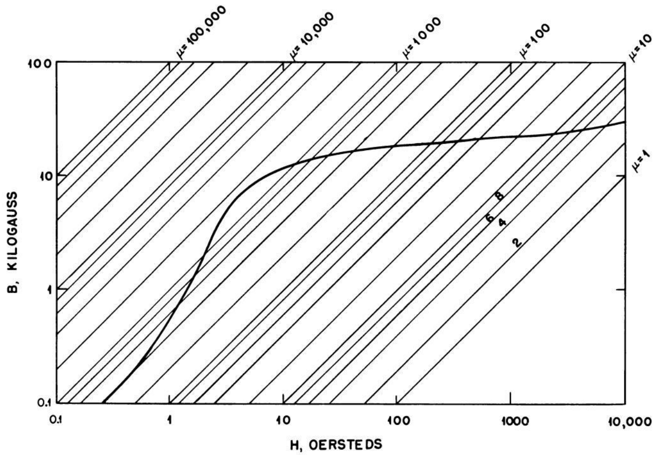
Fig. 1.5—Normal magnetization curve for SAE 1010 iron.
